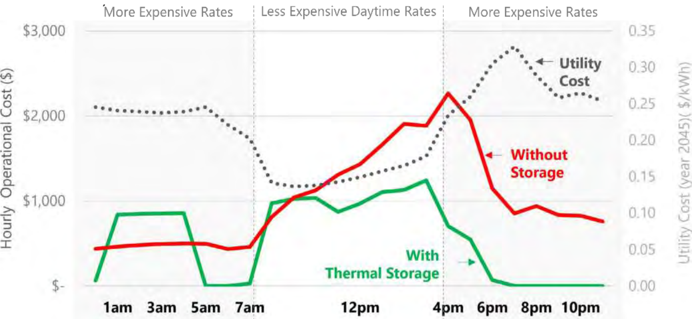
Hourly Energy Cost (September Day)
