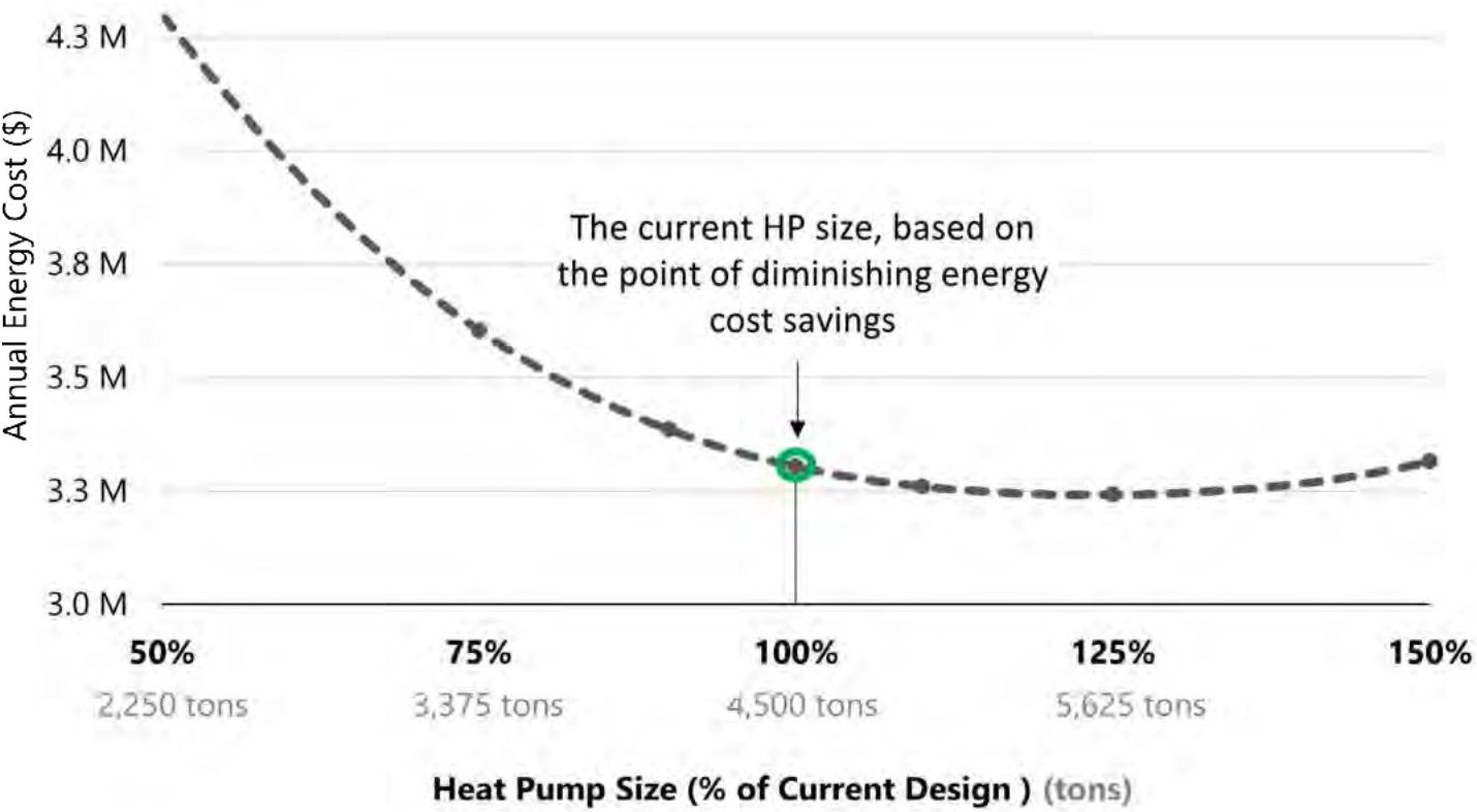
Heat Pump Size | Sensitivity Analysis
