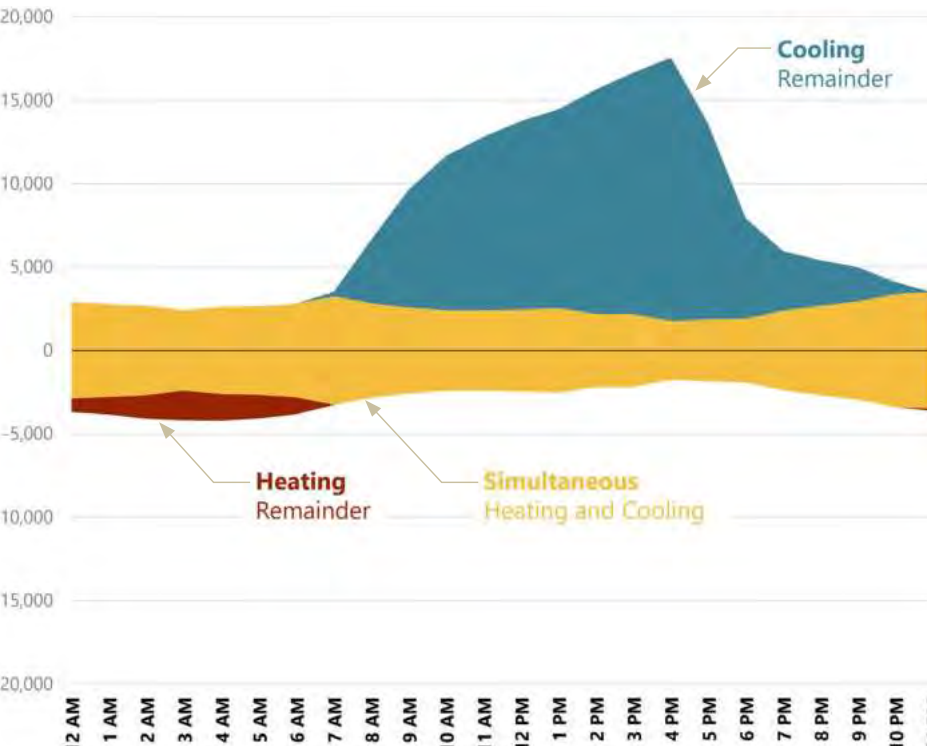
Typical Day Thermal Loads (kWh)
