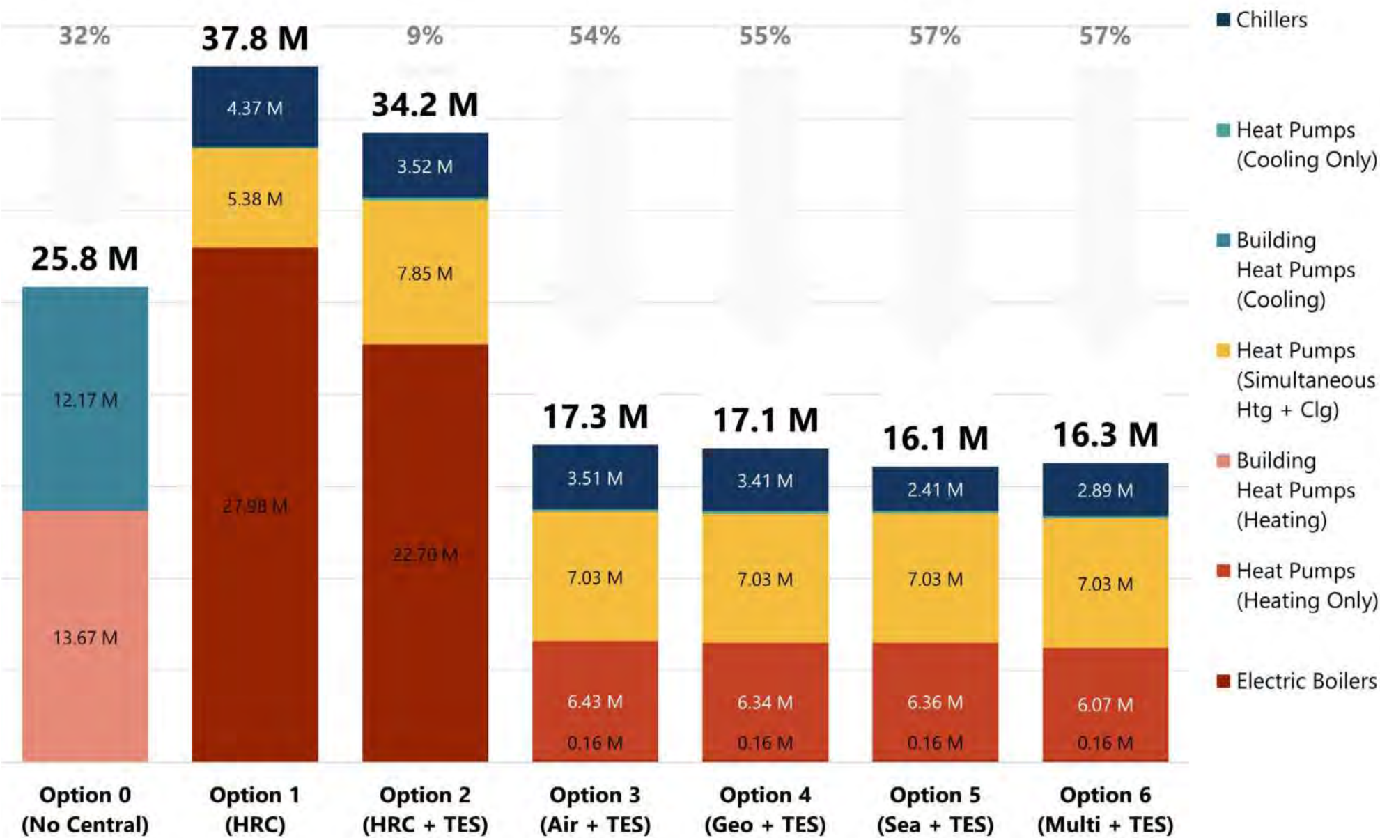
Simultaneous Thermal Loads (kWh/yr)
