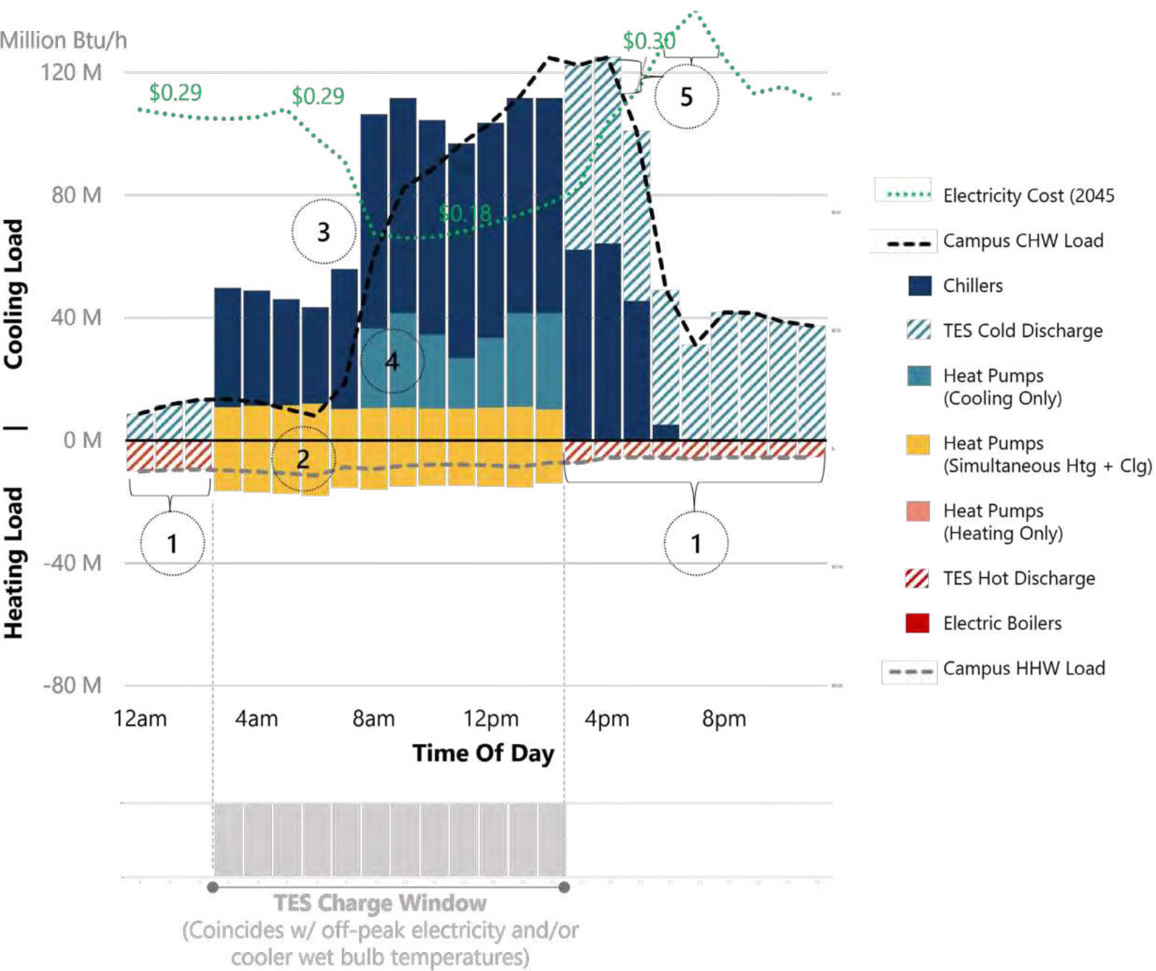
Load Profile by Equipment (Typical Late Summer Day | September)
