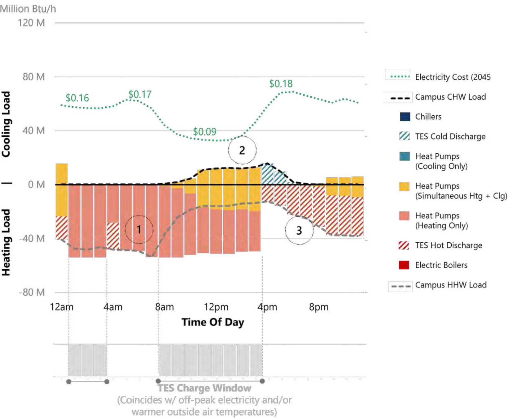
Load Profile by Equipment (Typical Winter Day | February)
