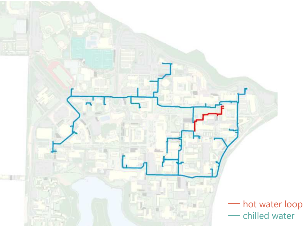
Current configuration of hydronic heating/cooling
