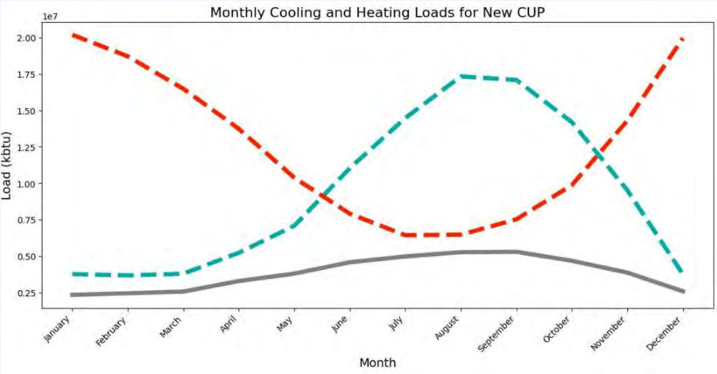
Heating vs Cooling Loads - New Central Utility Plant (CUP)
