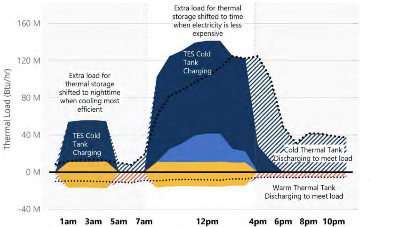
Thermal Load (September Day)
