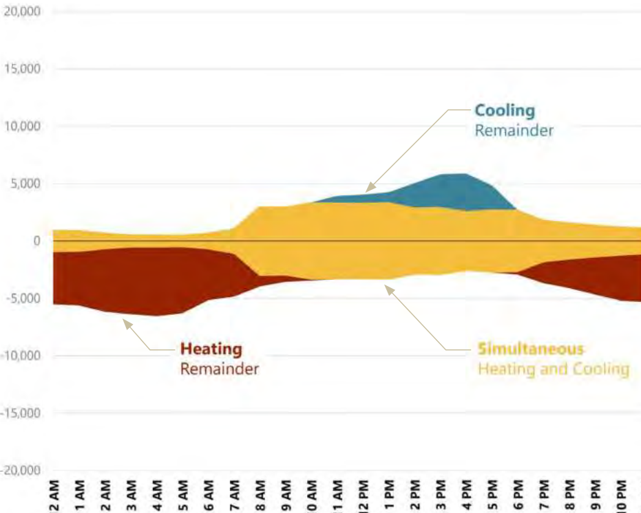
Typical Day Thermal Loads (kWh)
