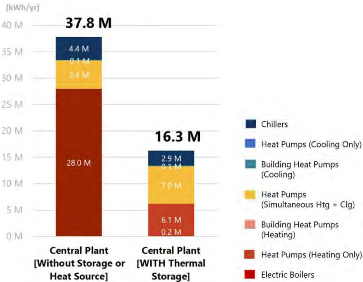
Energy Use By Equipment
