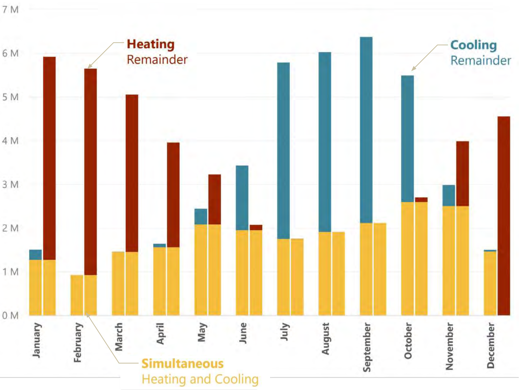
Monthly Thermal Loads (kWh)
